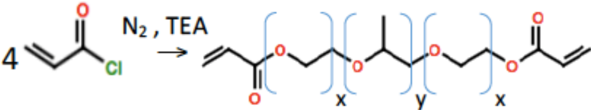
Acryloyl chloride
